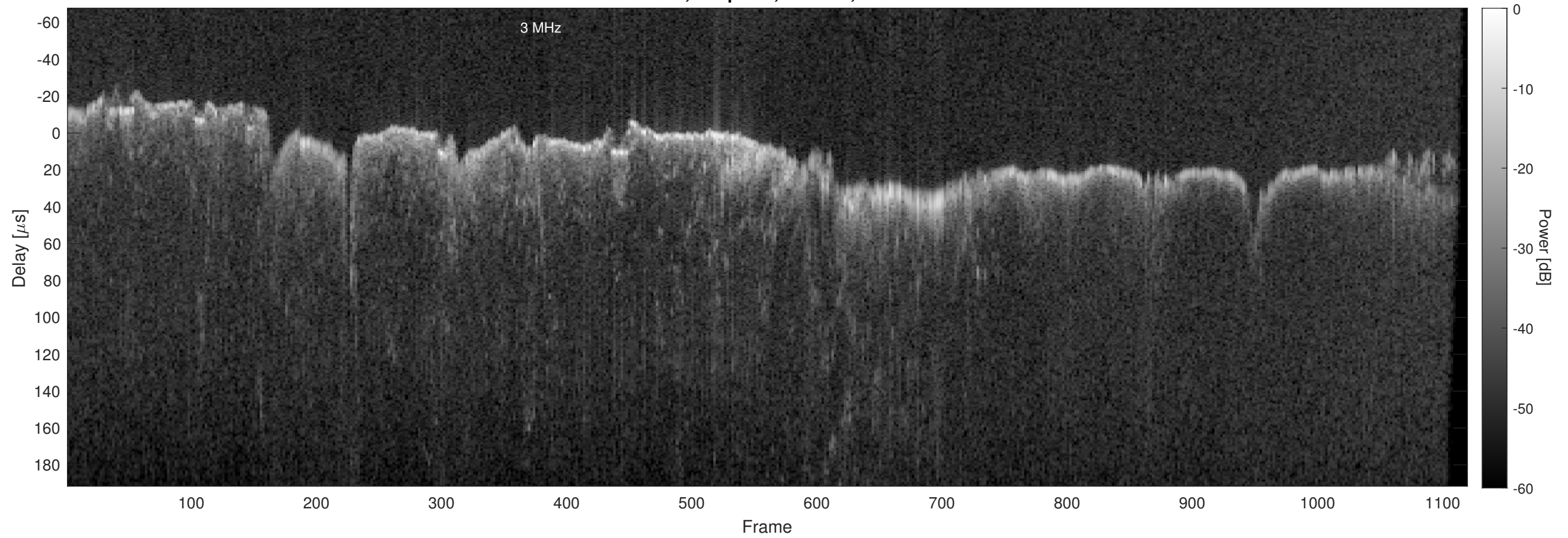
Orbit 12183, Chapman, Window, Channel 2
