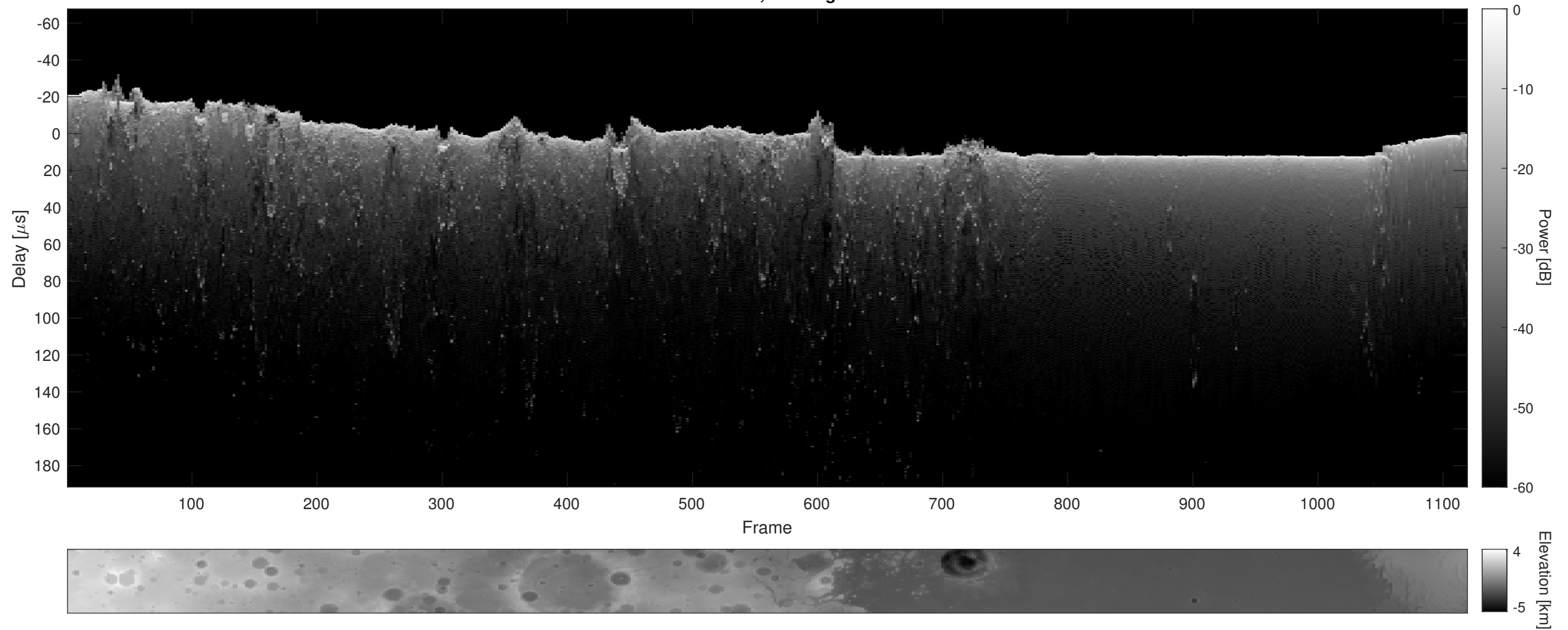
Orbit 12183, Cluttergram
