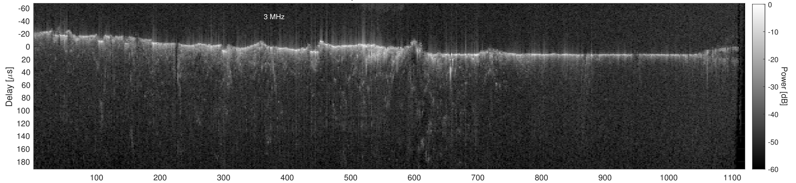
Orbit 12183, Cluttergram
