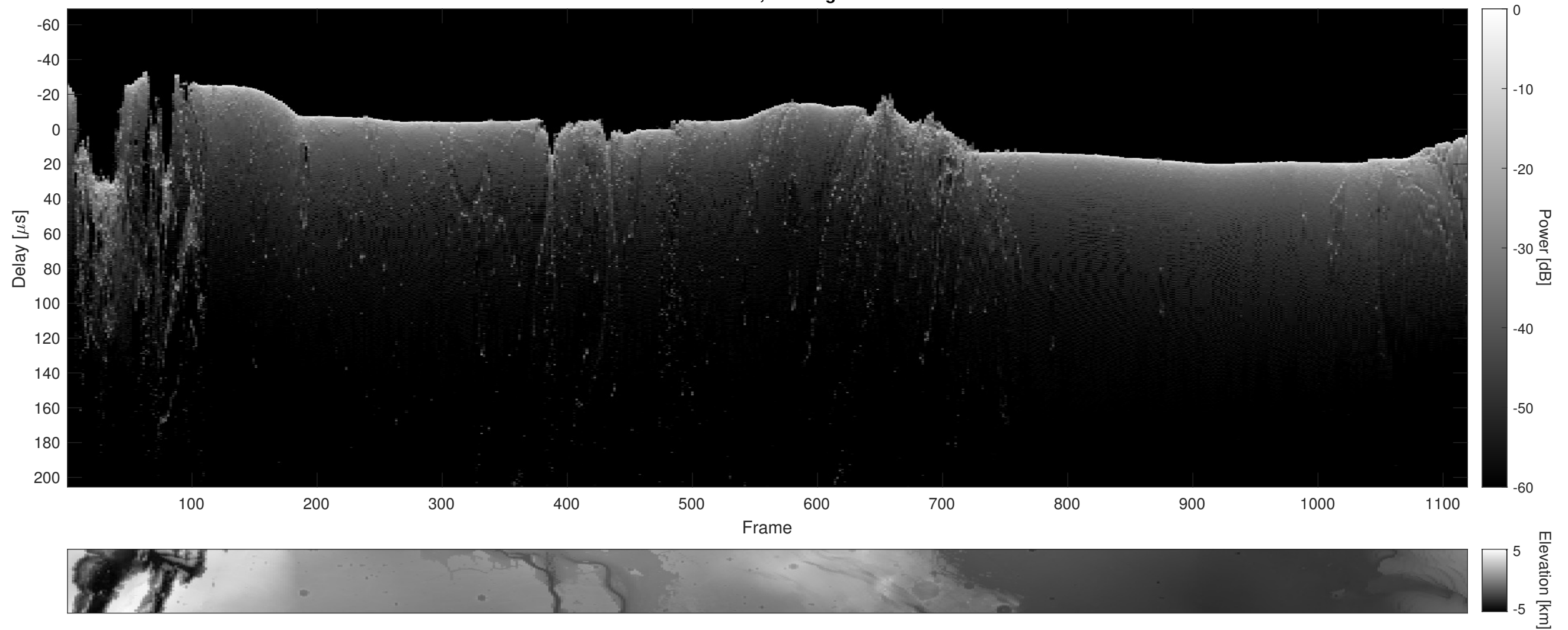
Orbit 12184, Cluttergram
