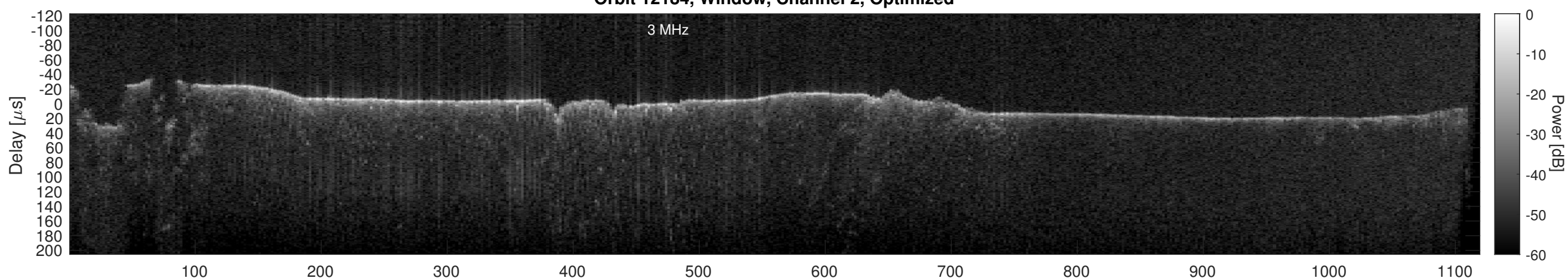
Orbit 12184, Cluttergram
