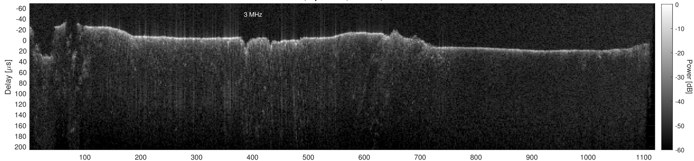
Orbit 12184, Cluttergram
