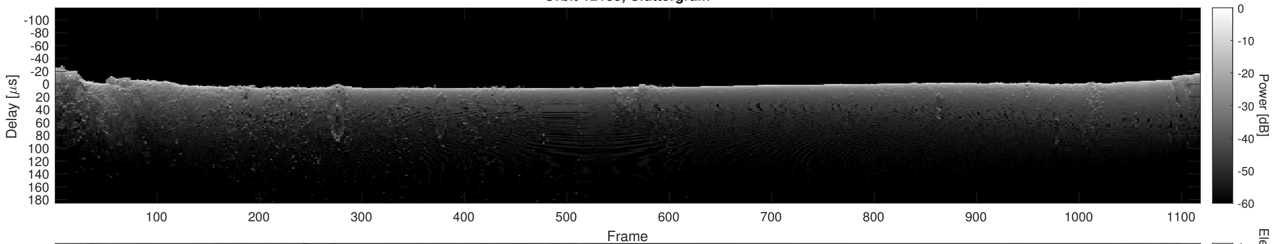
Orbit 12185, Cluttergram
