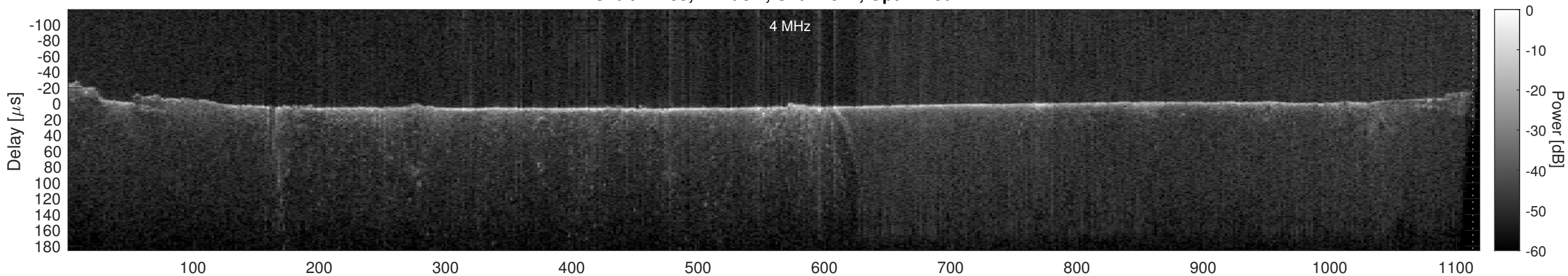
Orbit 12185, Cluttergram
