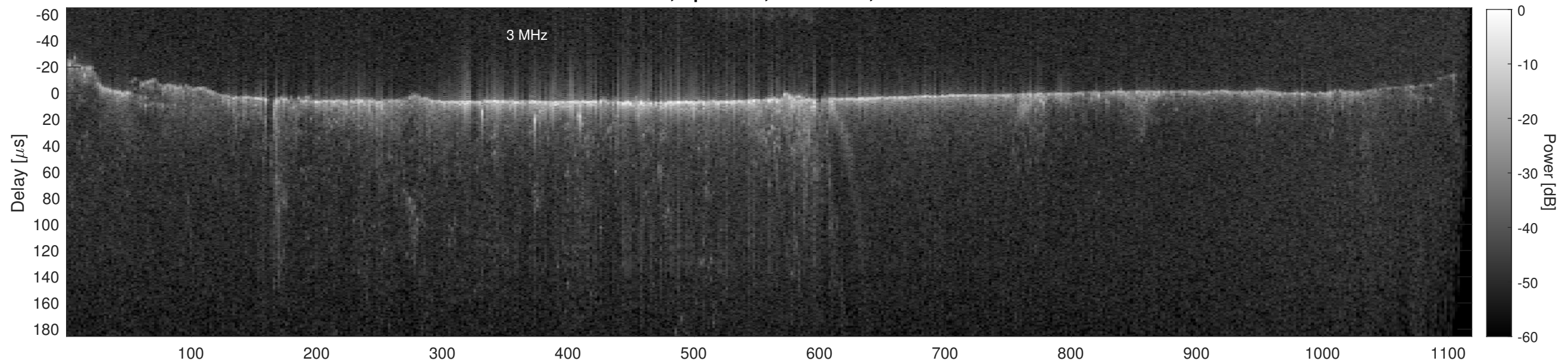
Orbit 12185, Cluttergram
