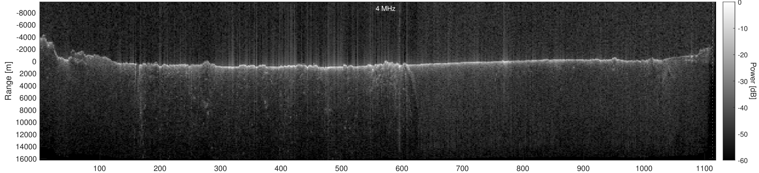
Orbit 12185, Optimized, No Window, Depth-Corrected, Channel 2
