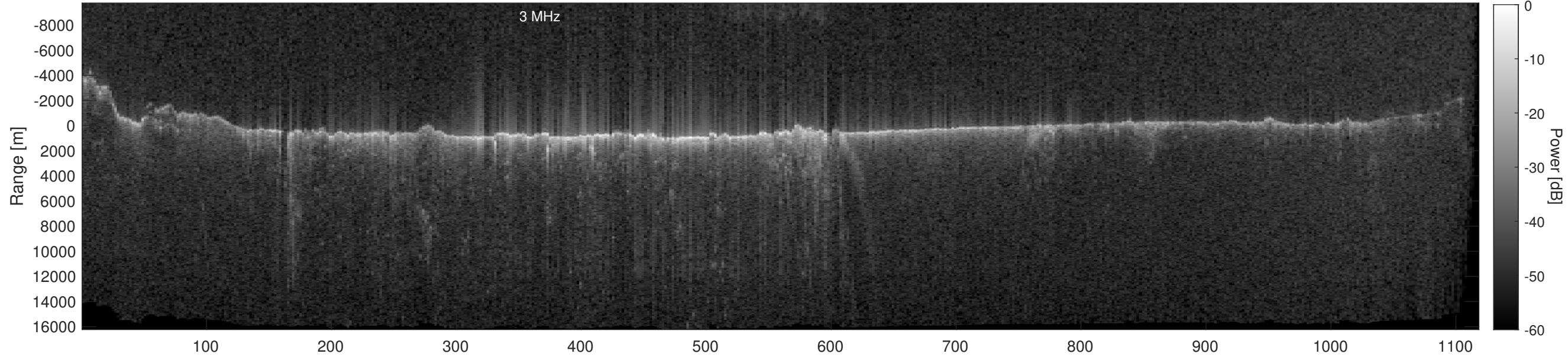
Orbit 12185, Depth-Corrected Cluttergram
