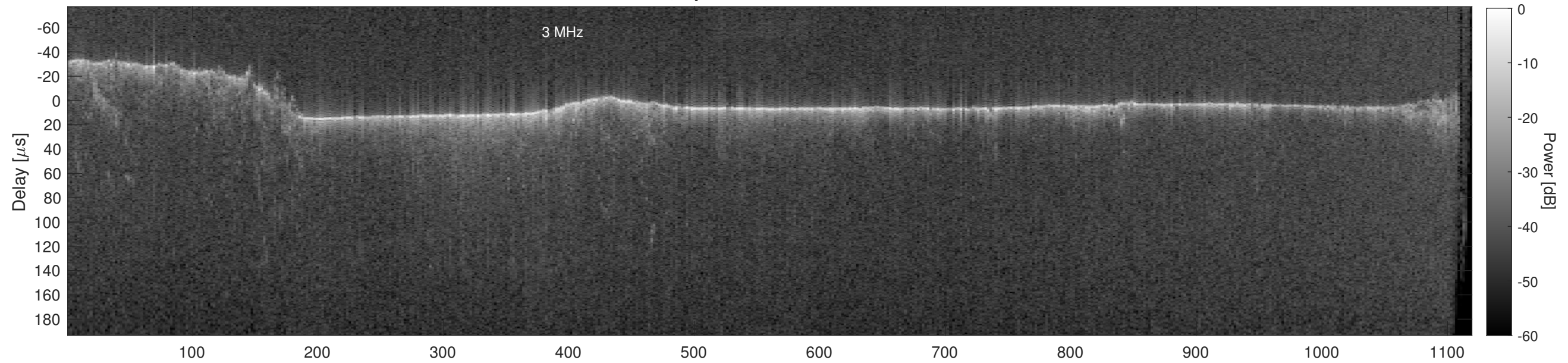
Orbit 12186, Cluttergram
