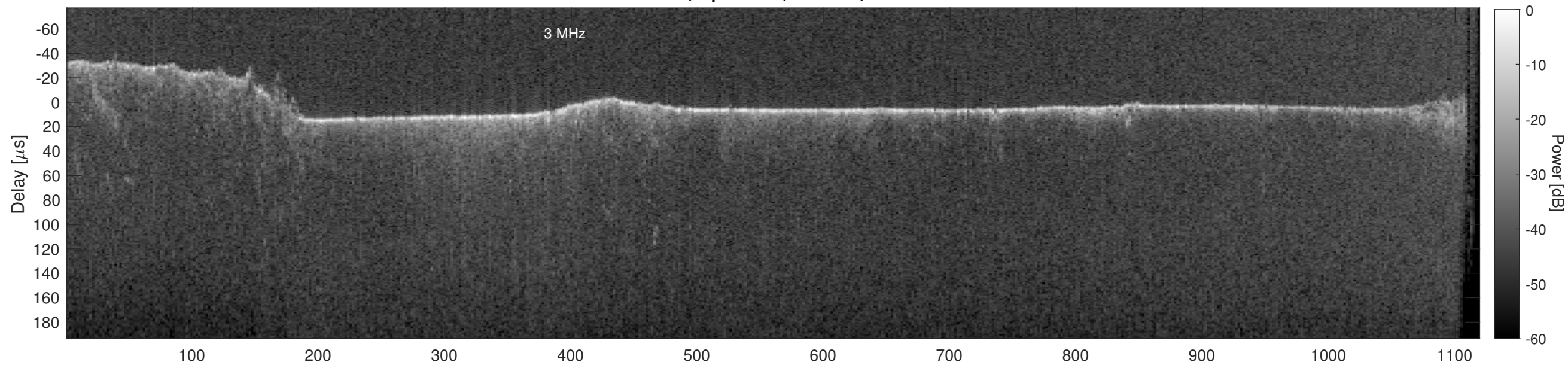
Orbit 12186, Cluttergram
