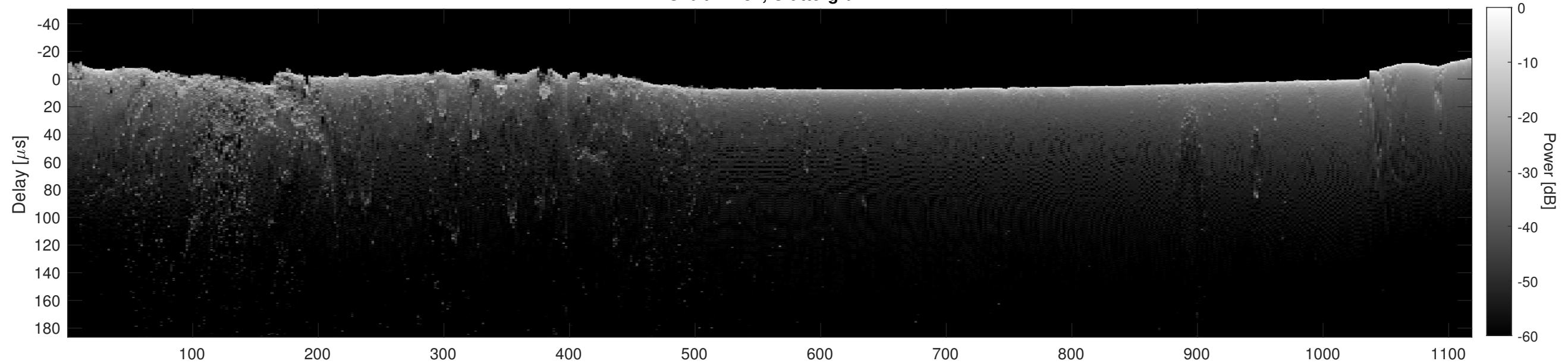
Orbit 12187, Cluttergram
