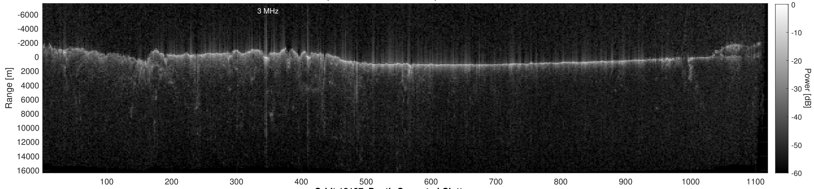
Orbit 12187, Depth-Corrected Cluttergram
