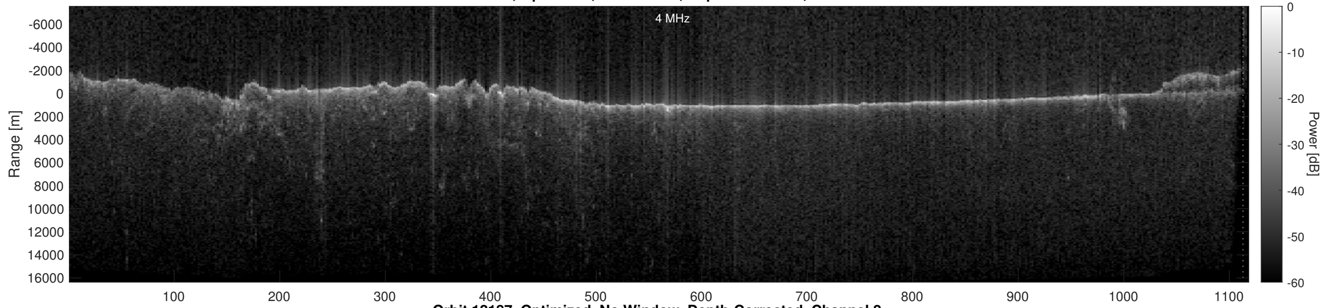
Orbit 12187, Optimized, No Window, Depth-Corrected, Channel 2
