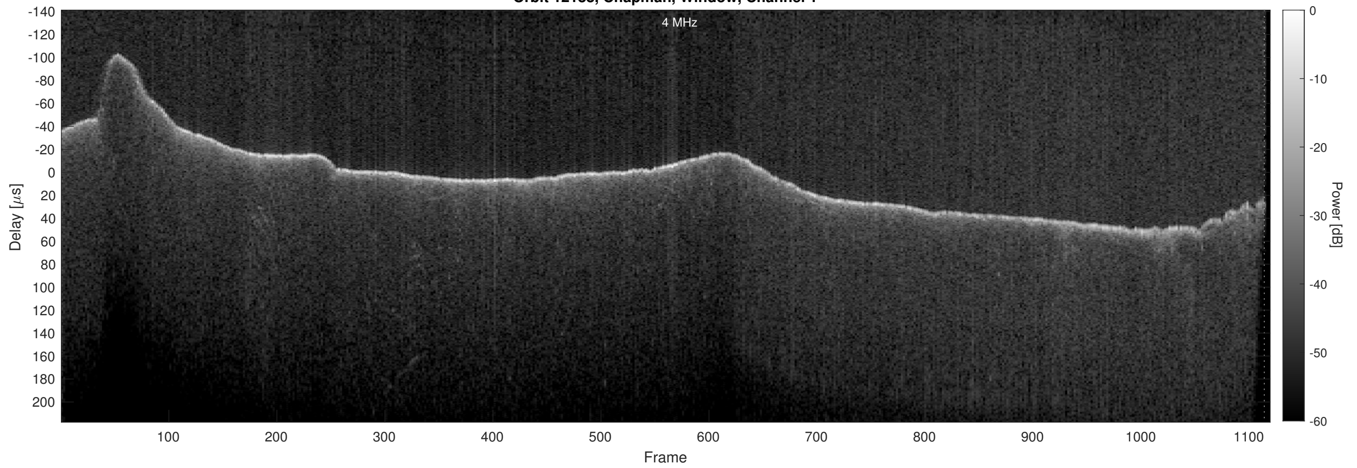
Orbit 12188, Chapman, Window, Channel 2
