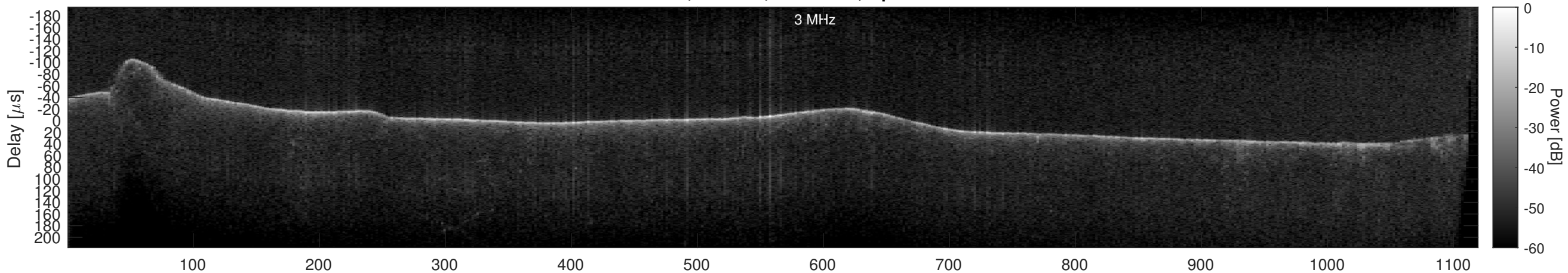
Orbit 12188, Cluttergram
