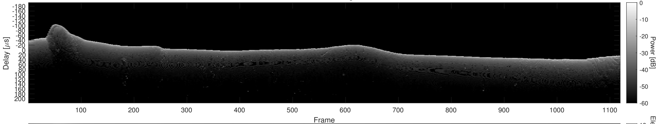
Orbit 12188, Cluttergram
