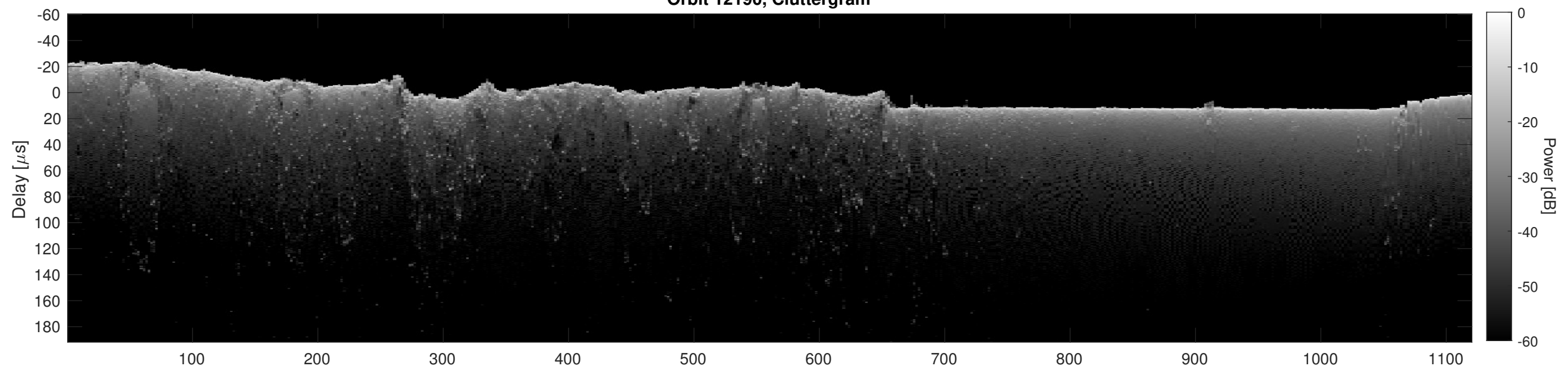
Orbit 12190, Cluttergram
