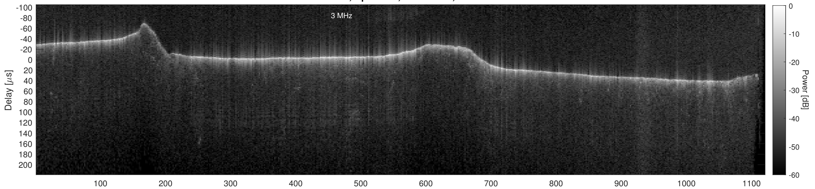
Orbit 12195, Cluttergram
