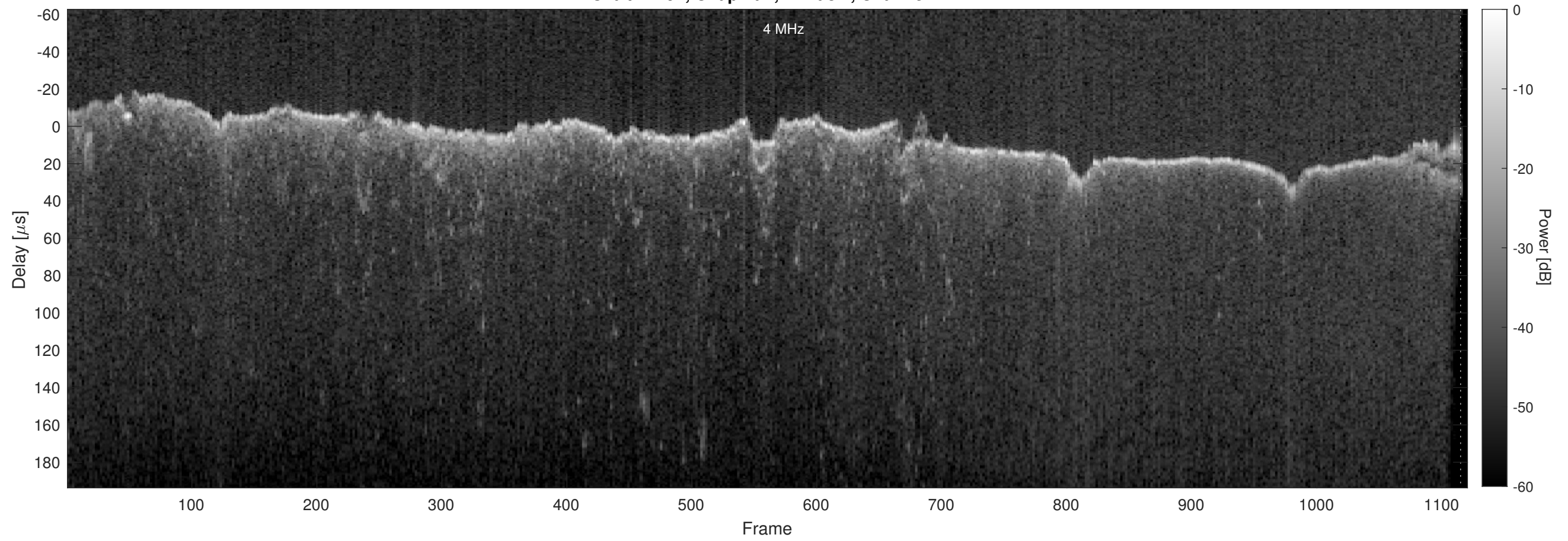
Orbit 12197, Chapman, Window, Channel 2
