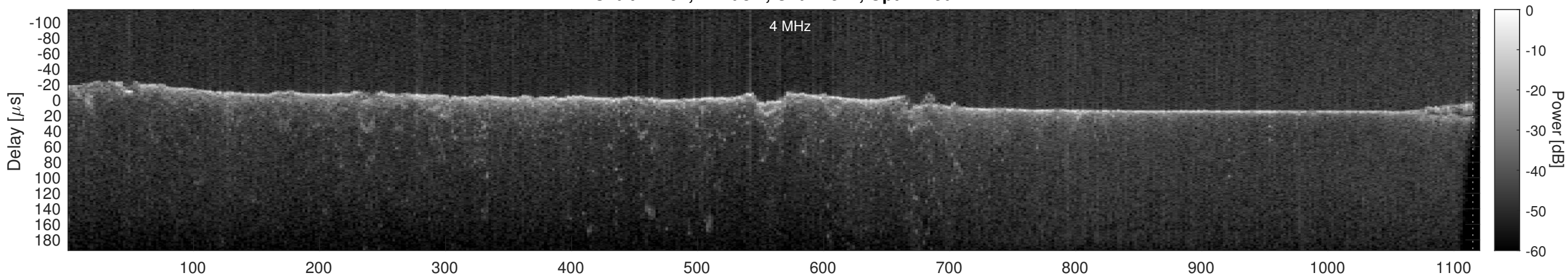
Orbit 12197, Cluttergram
