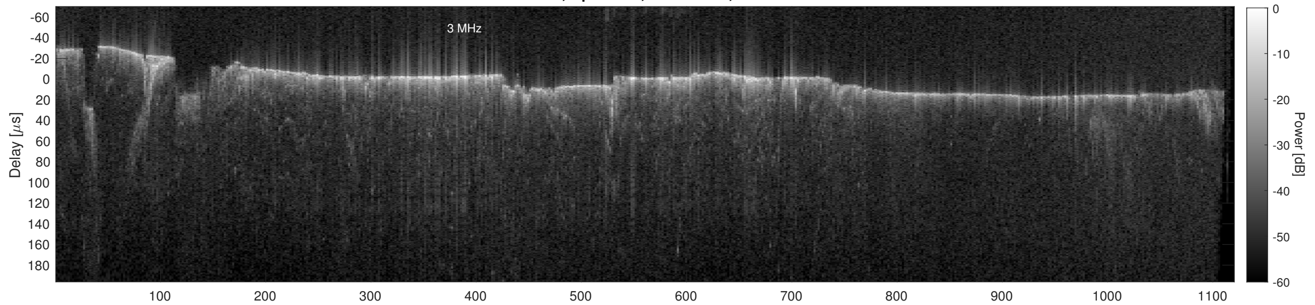
Orbit 12198, Cluttergram
