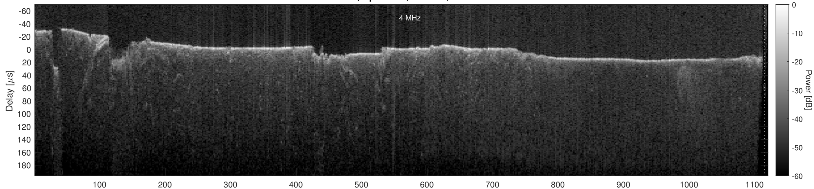
Orbit 12198, Optimized, Window, Channel 2
