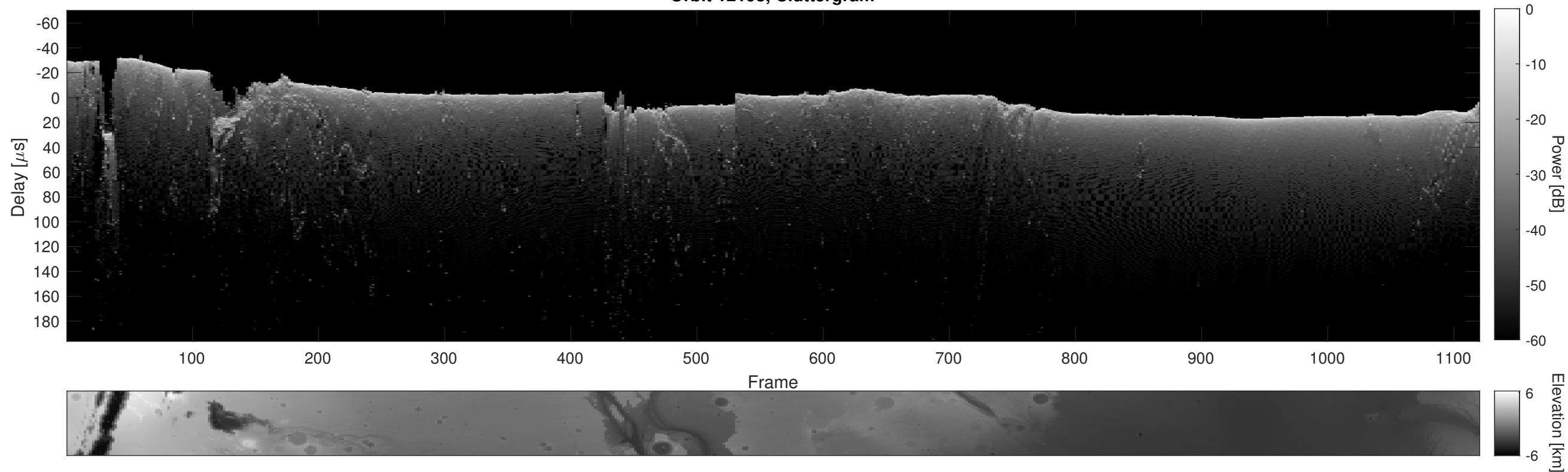
Orbit 12198, Cluttergram
