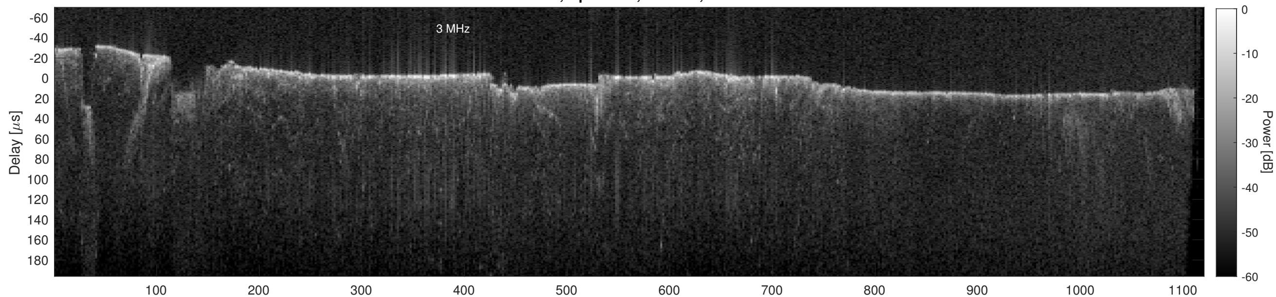
Orbit 12198, Cluttergram
