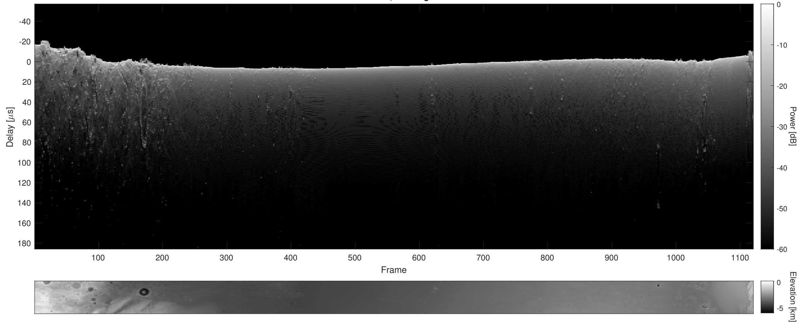
Orbit 12199, Cluttergram
