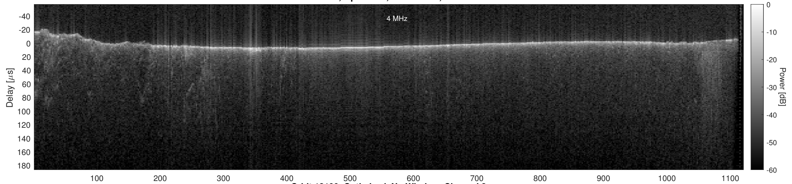
Orbit 12199, Optimized, No Window, Channel 2
