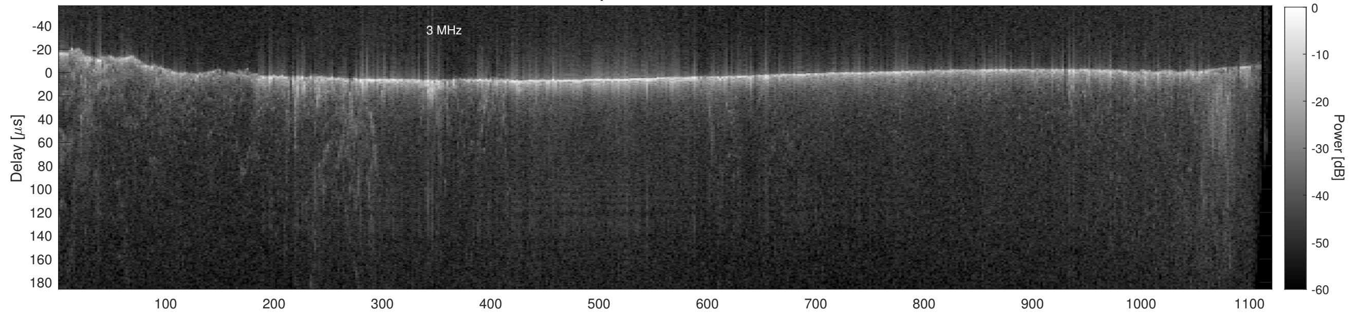
Orbit 12199, Cluttergram
