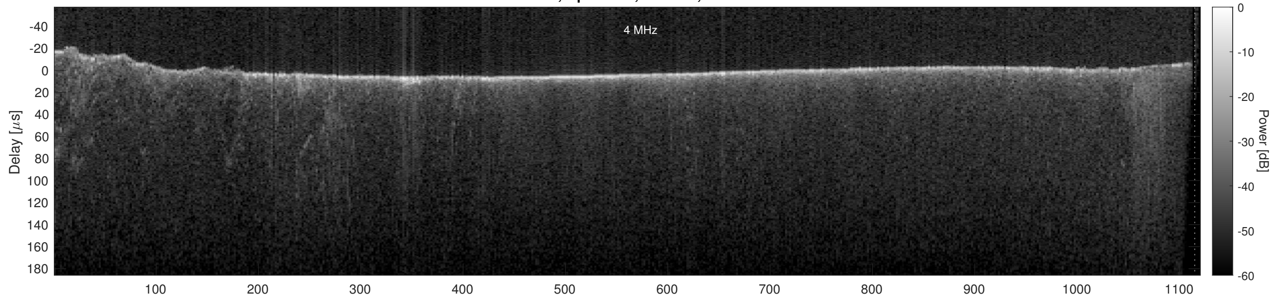
Orbit 12199, Optimized, Window, Channel 2
