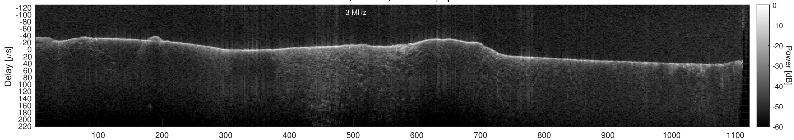
Orbit 12202, Cluttergram
