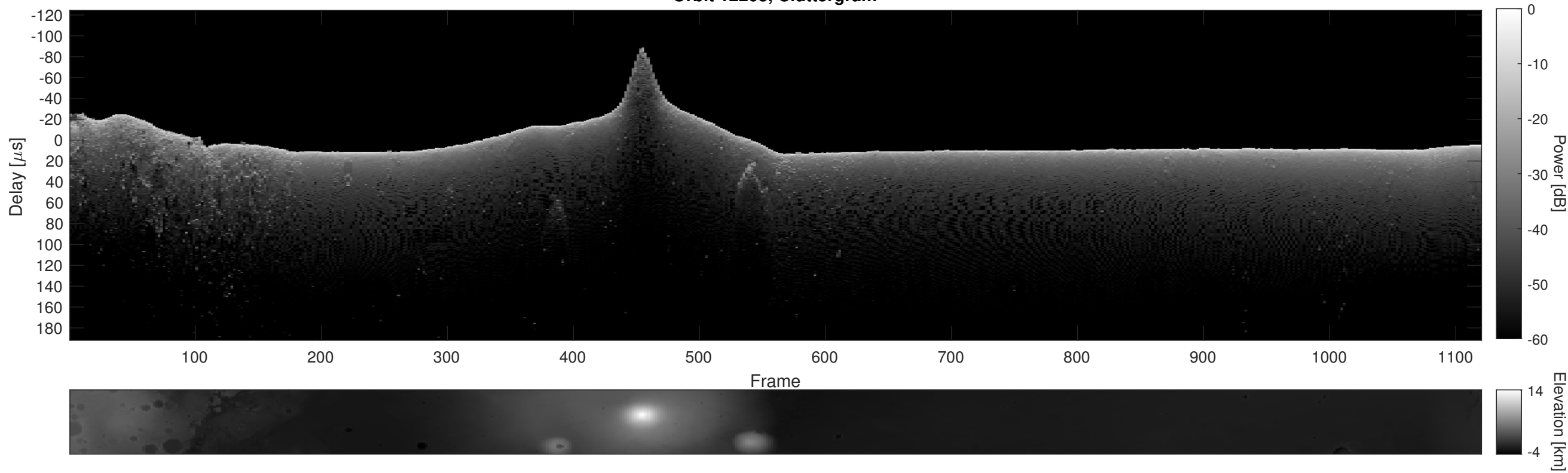
Orbit 12203, Cluttergram
