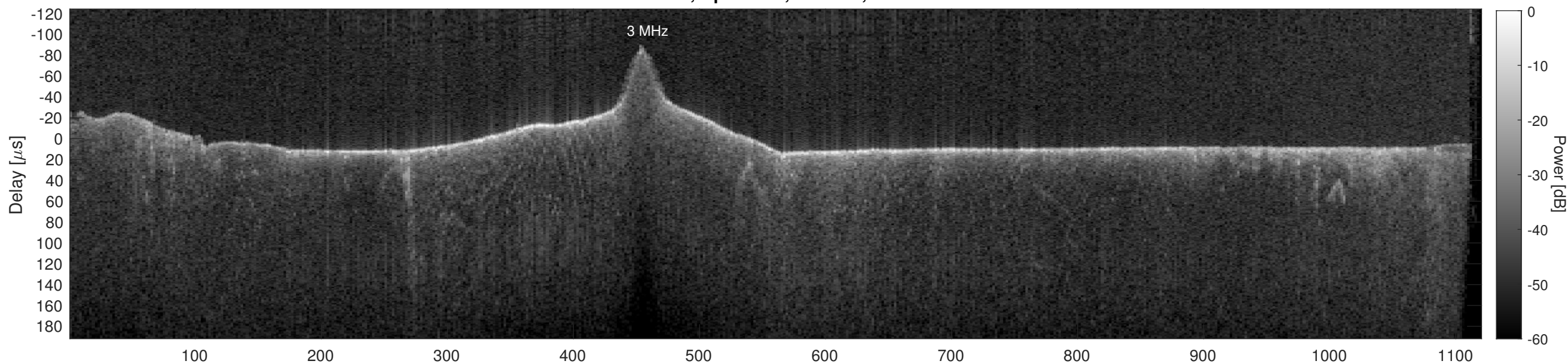
Orbit 12203, Cluttergram
