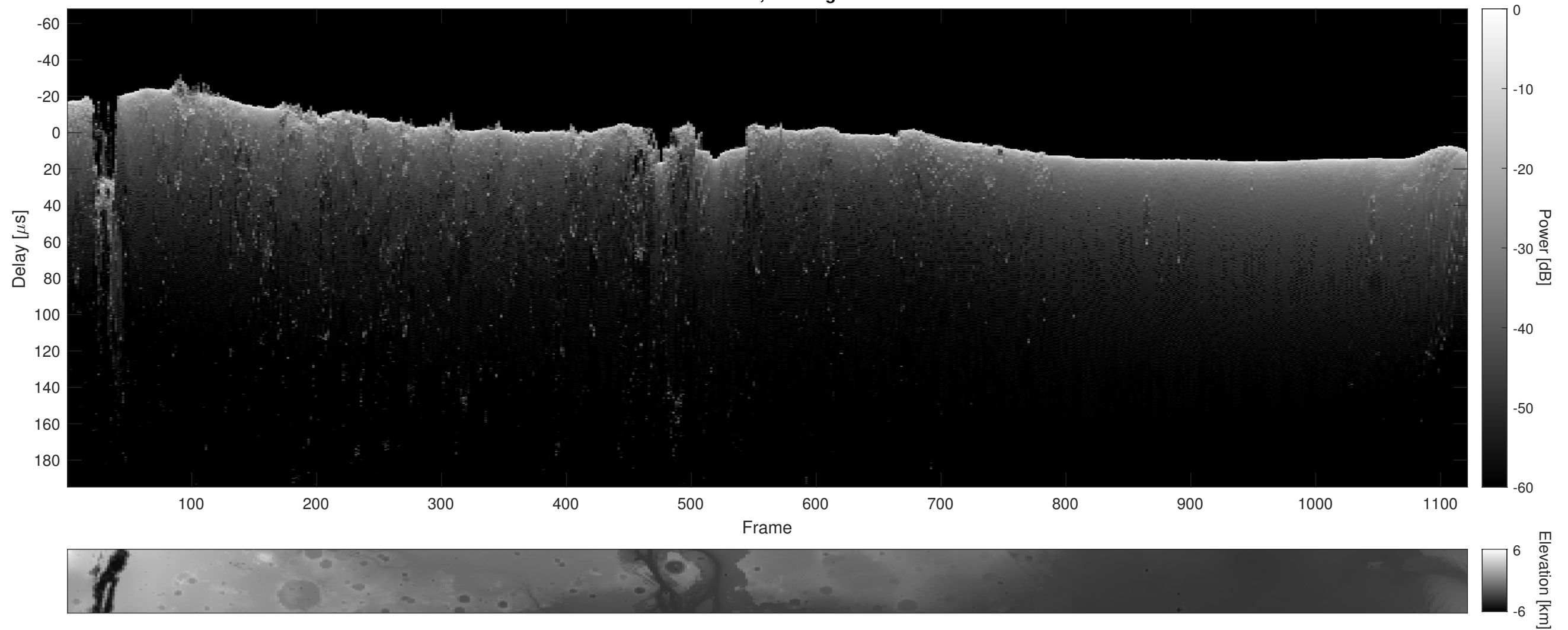
Orbit 12205, Cluttergram
