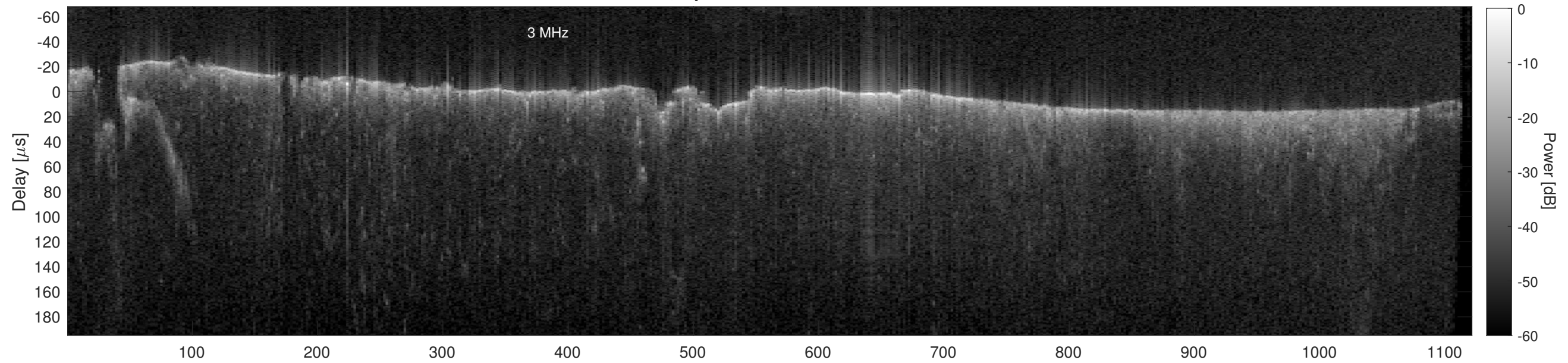
Orbit 12205, Cluttergram
