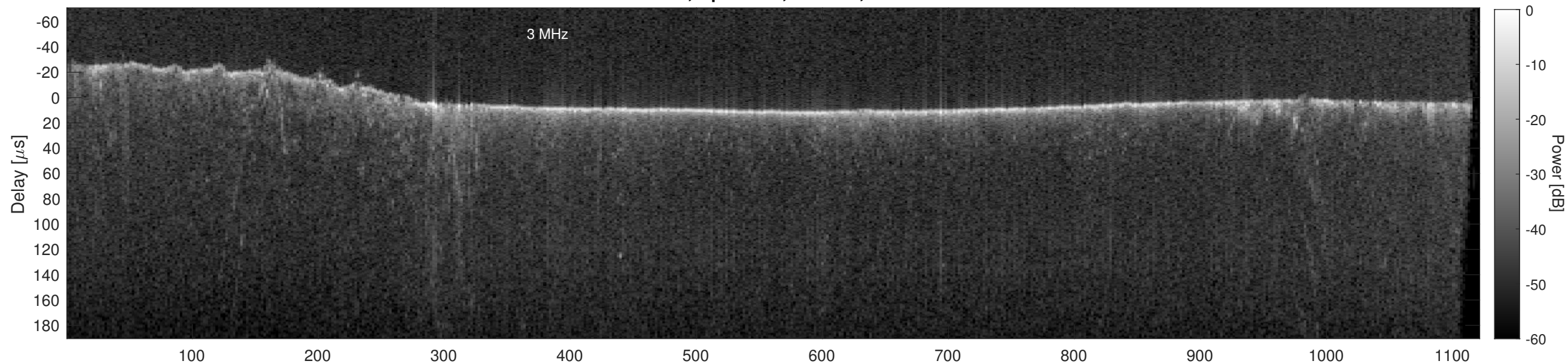
Orbit 12207, Cluttergram
