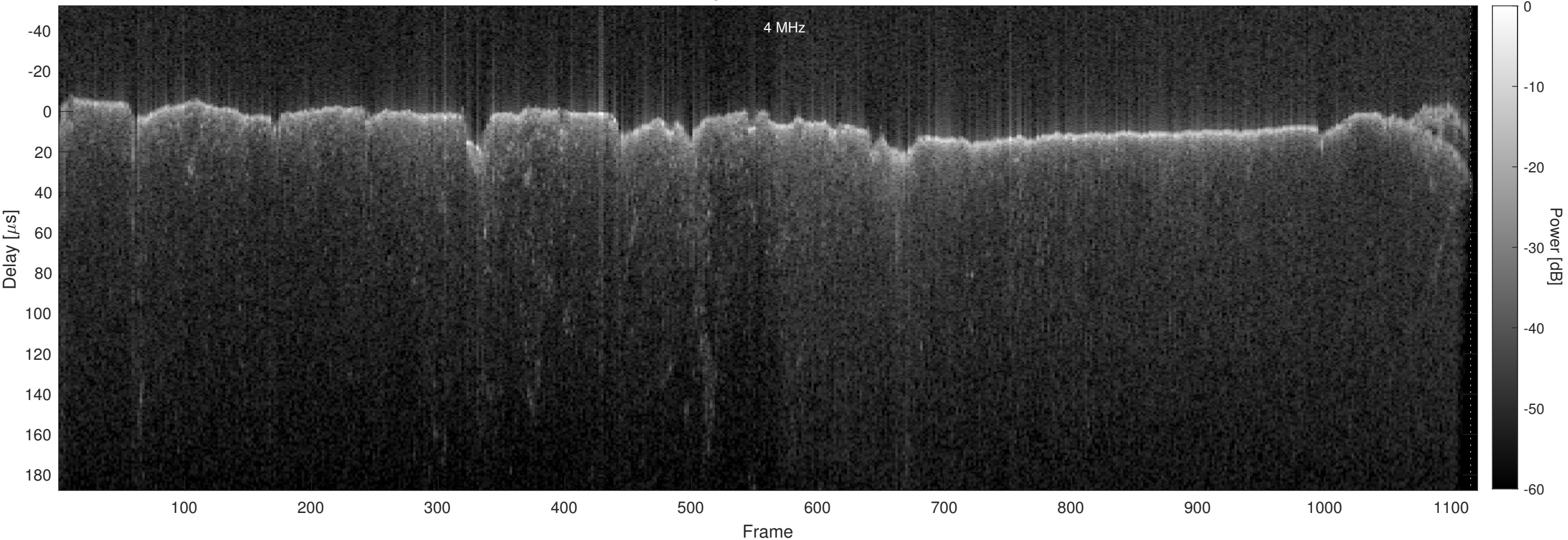
Orbit 12208, Chapman, No Window, Channel 2
