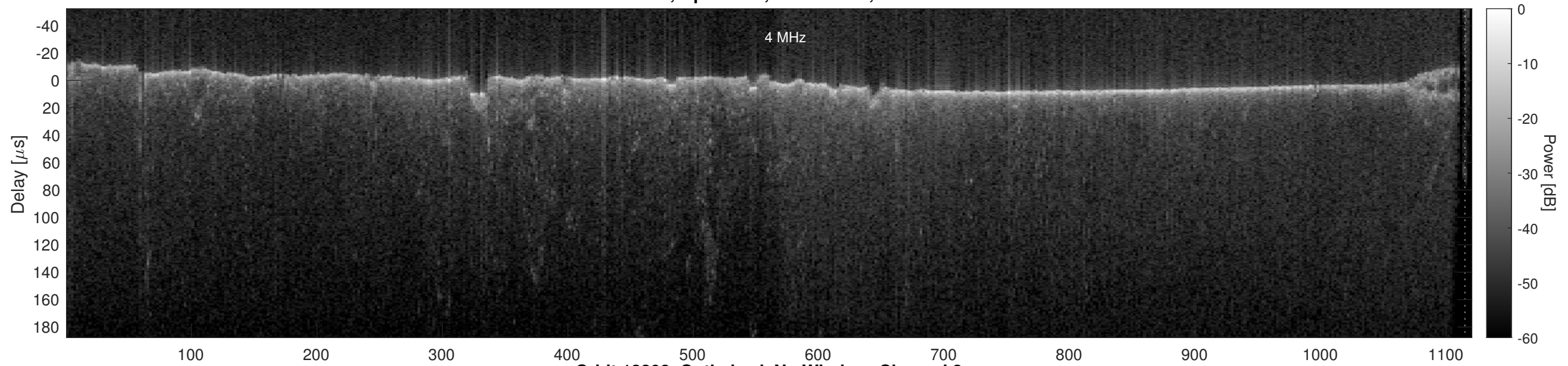
Orbit 12208, Optimized, No Window, Channel 2
