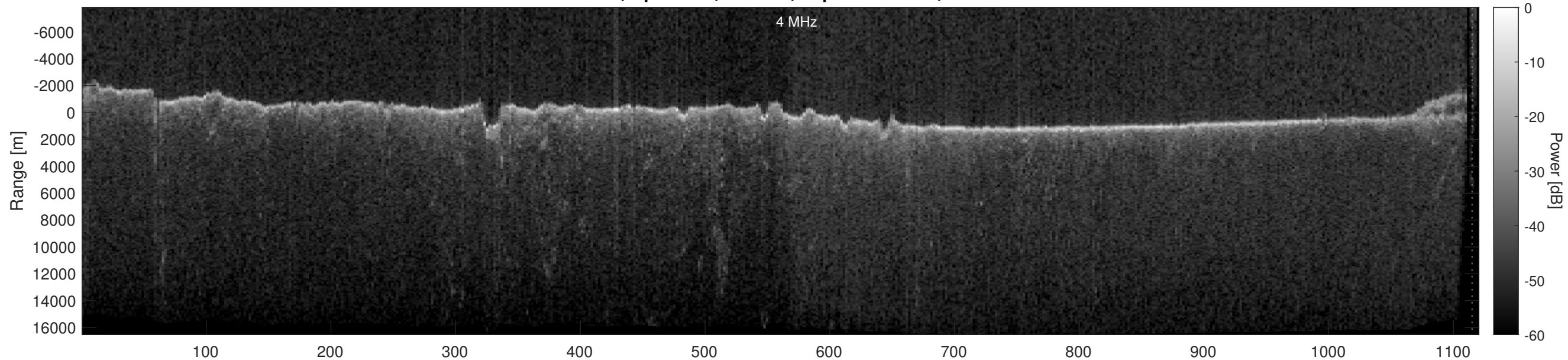
Orbit 12208, Optimized, Window, Depth-Corrected, Channel 2
