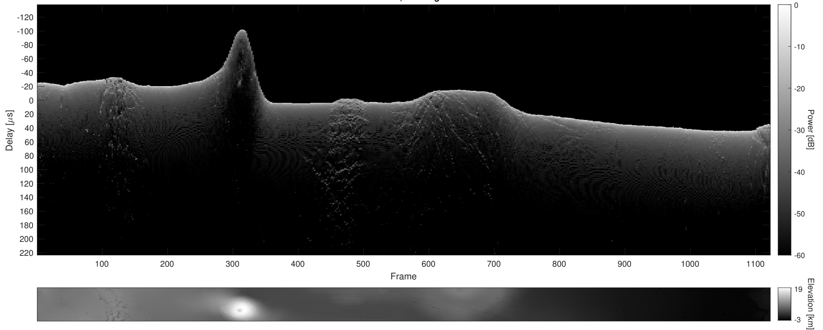
Orbit 12209, Cluttergram
