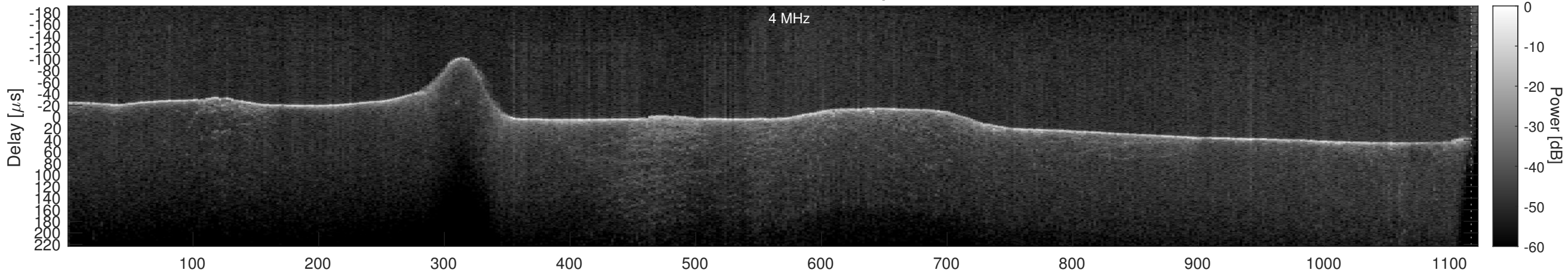
Orbit 12209, Cluttergram
