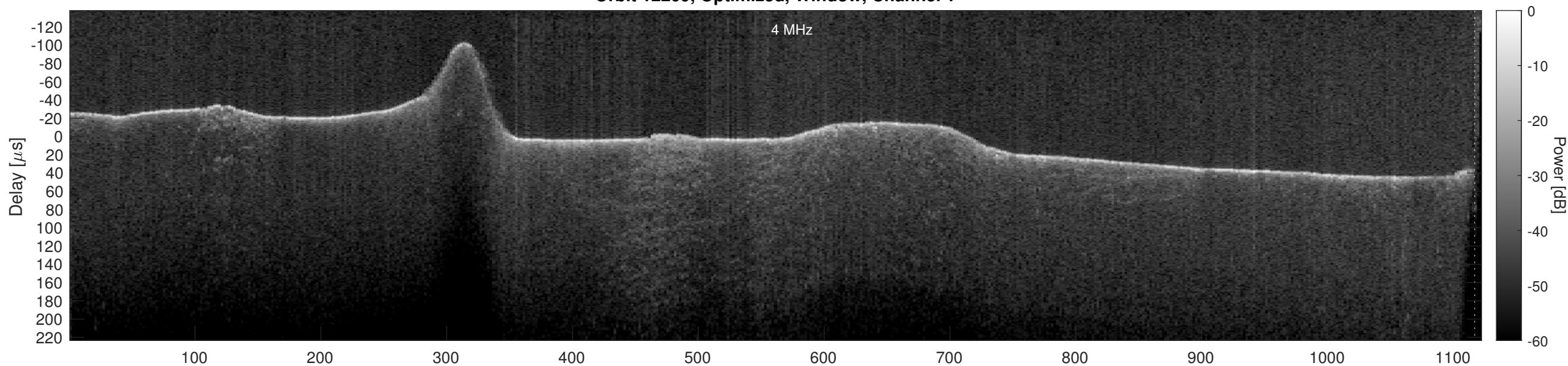
Orbit 12209, Optimized, Window, Channel 2
