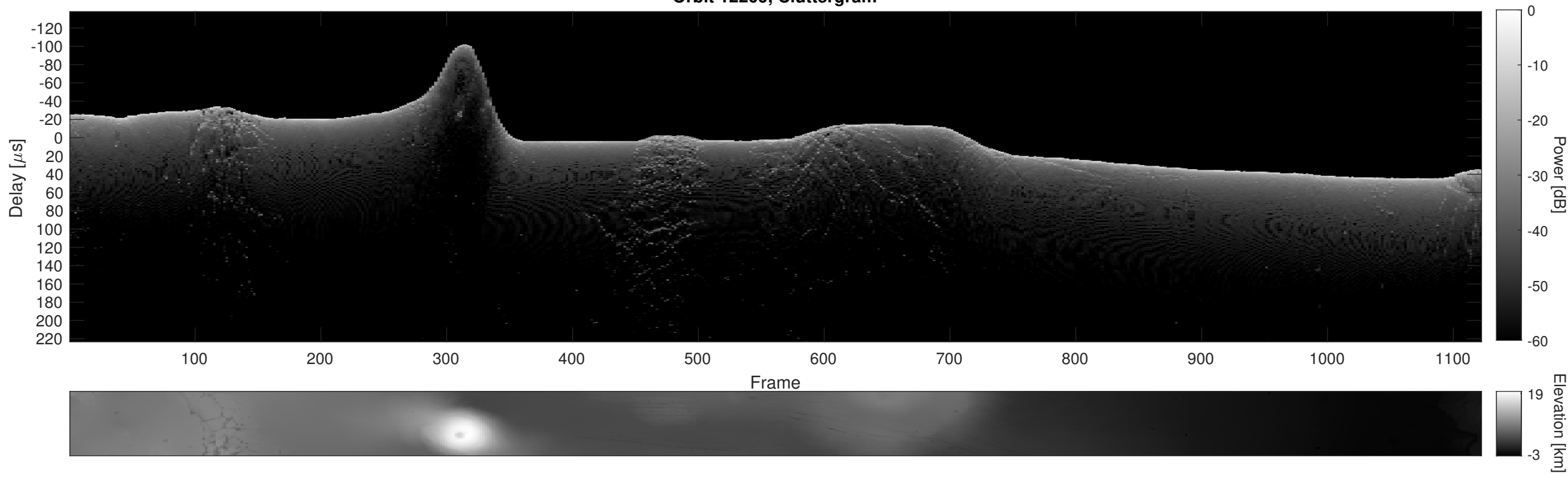
Orbit 12209, Cluttergram
