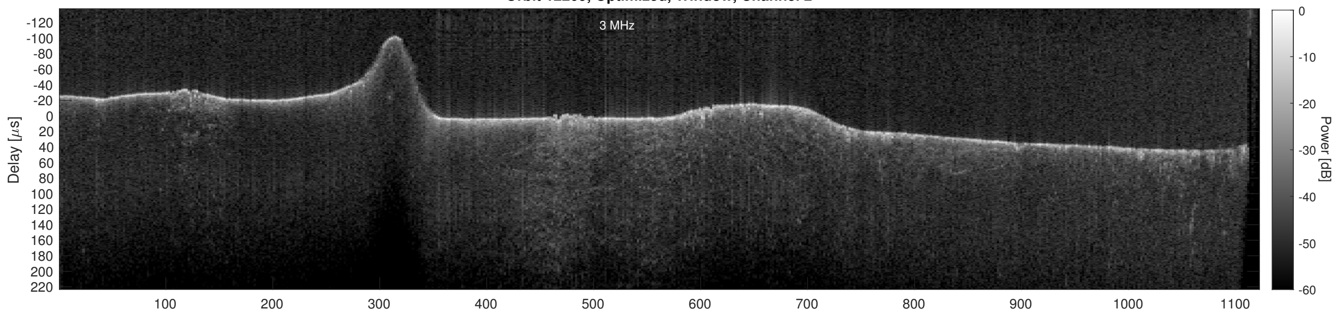
Orbit 12209, Cluttergram
