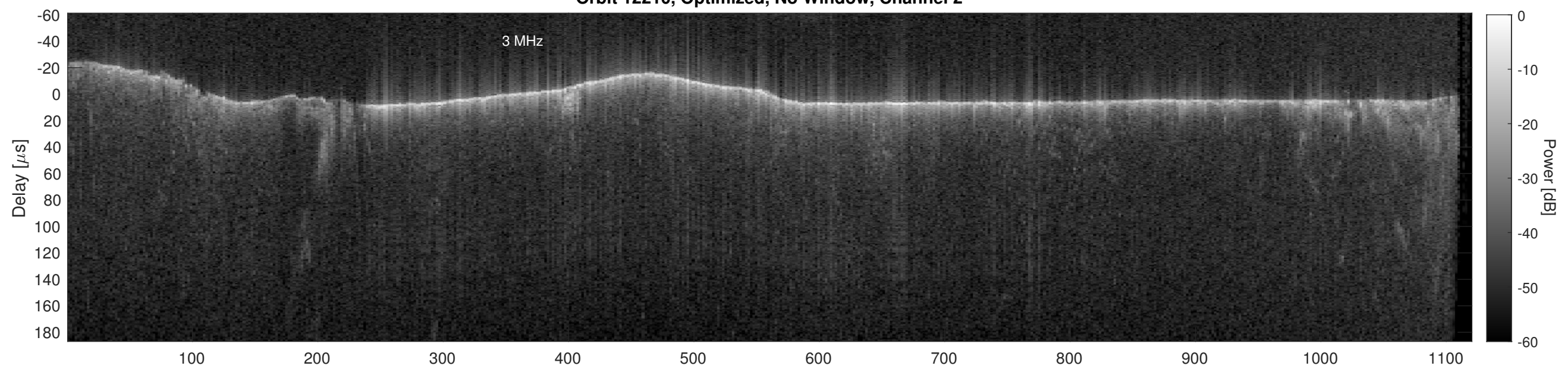
Orbit 12210, Cluttergram
