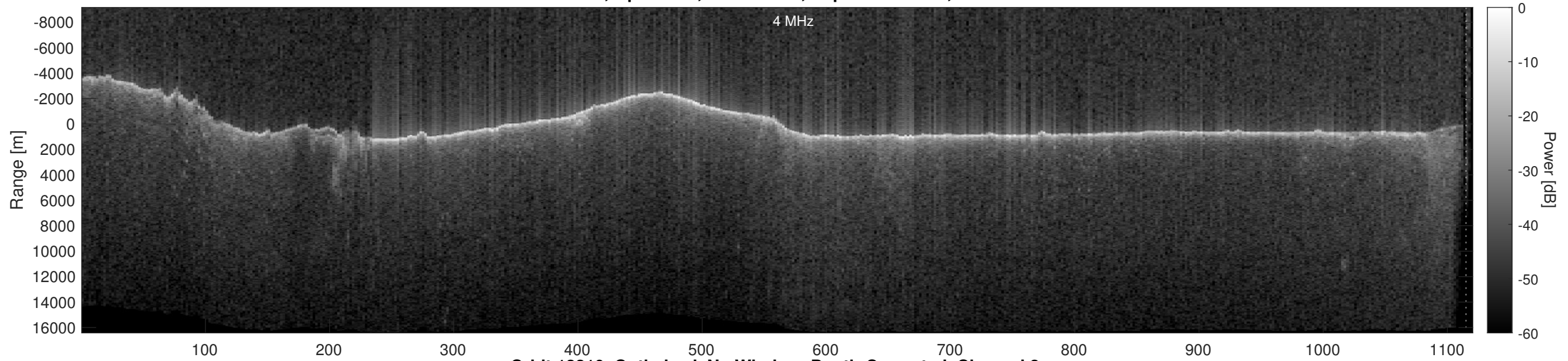
Orbit 12210, Optimized, No Window, Depth-Corrected, Channel 2
