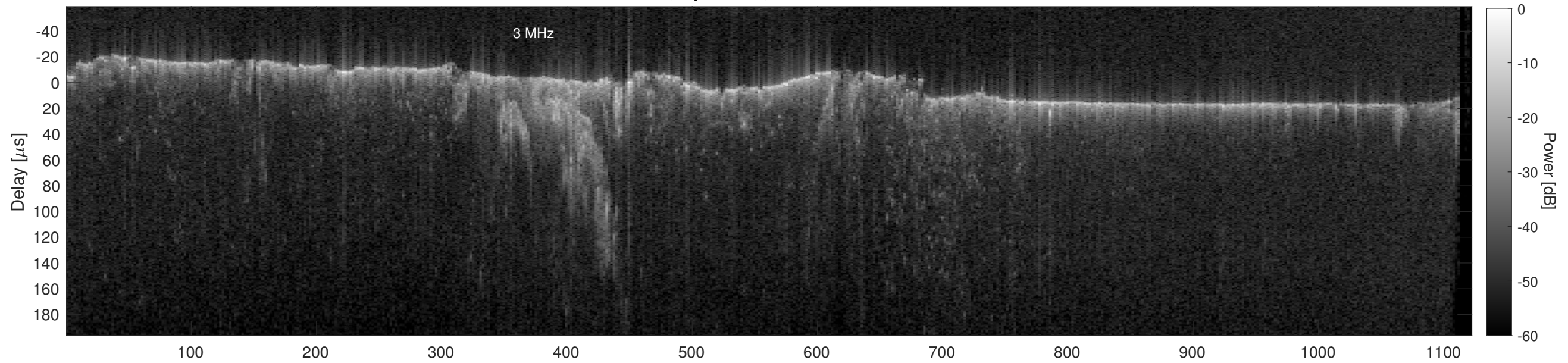
Orbit 12211, Cluttergram
