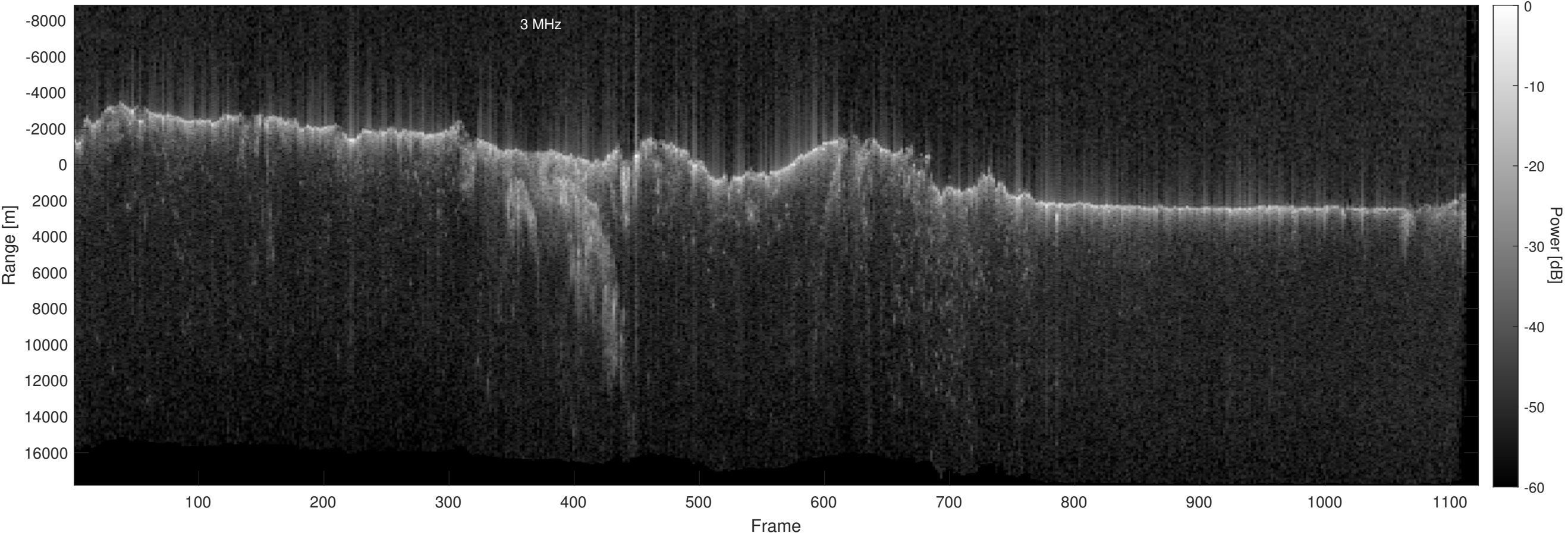
Orbit 12211, Optimized, No Window, Depth-Corrected, Channel 2
