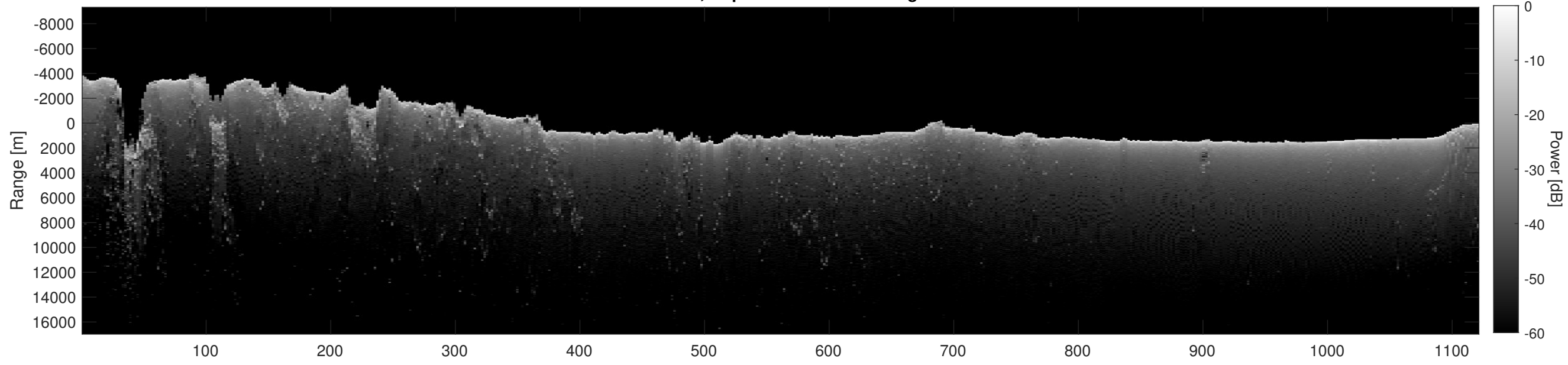
Orbit 12212, Depth-Corrected Cluttergram
