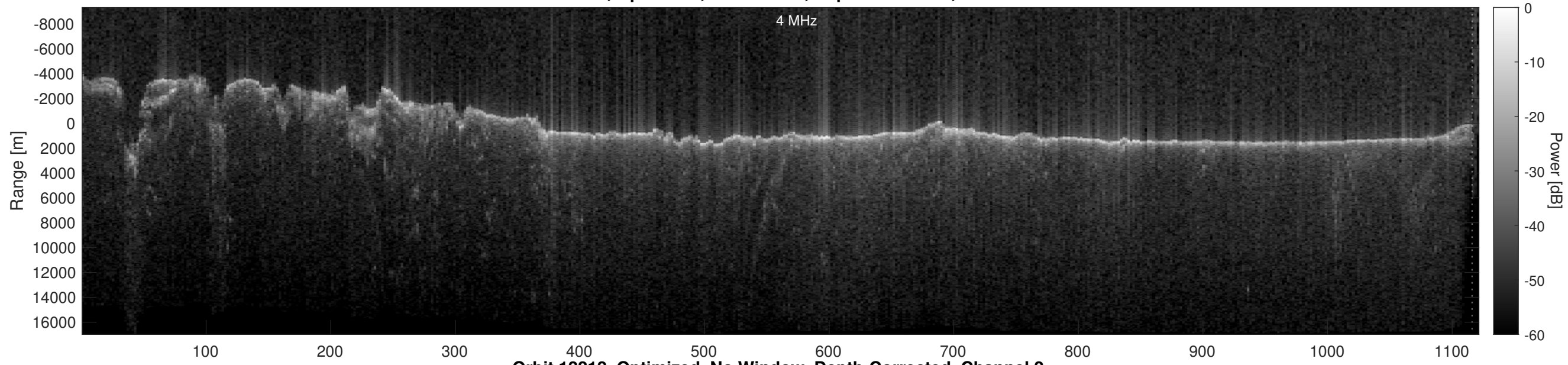
Orbit 12212, Optimized, No Window, Depth-Corrected, Channel 2
