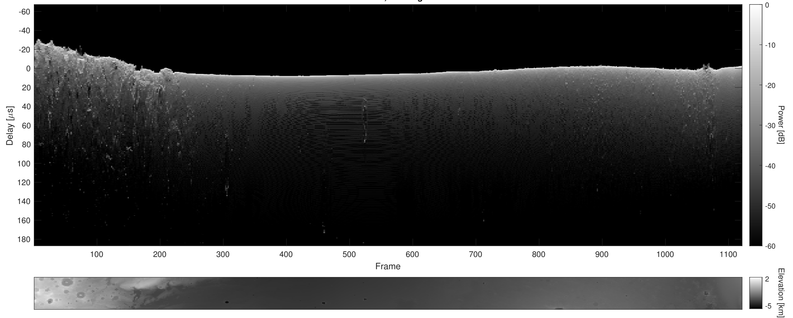
Orbit 12213, Cluttergram
