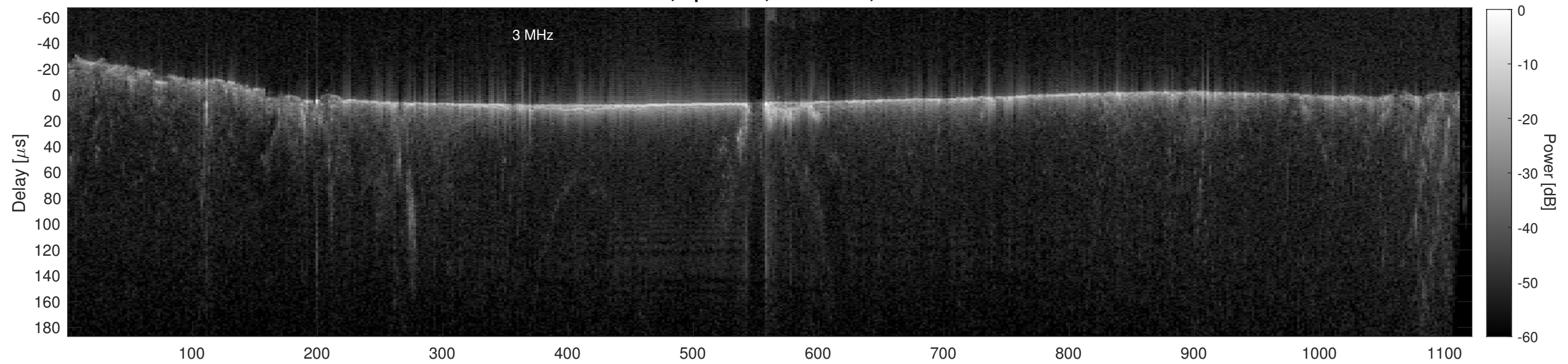
Orbit 12213, Cluttergram
