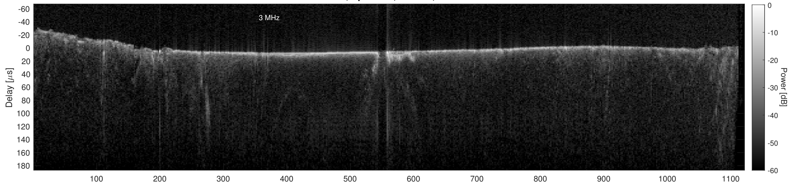
Orbit 12213, Cluttergram
