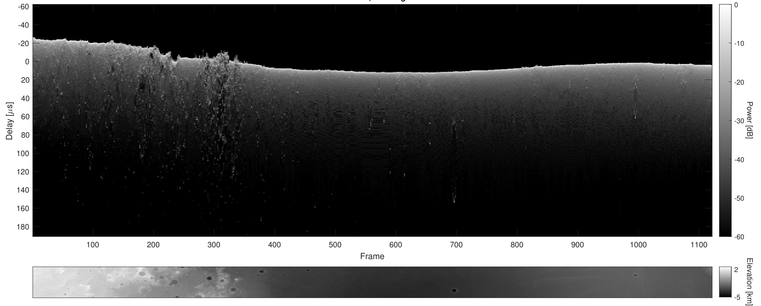
Orbit 12214, Cluttergram
