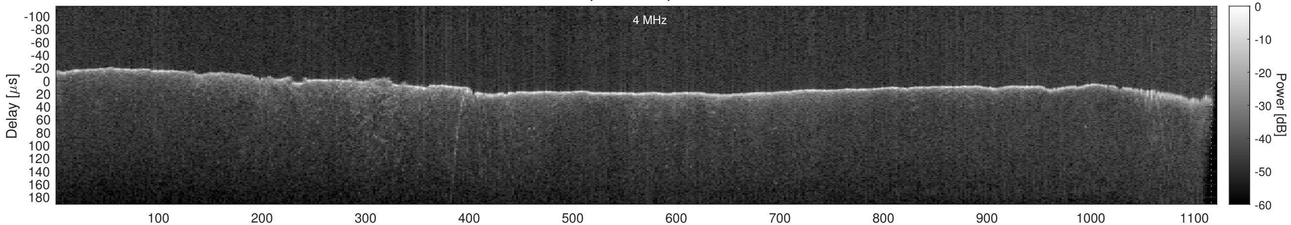
Orbit 12214, Window, Channel 1, Chapman
