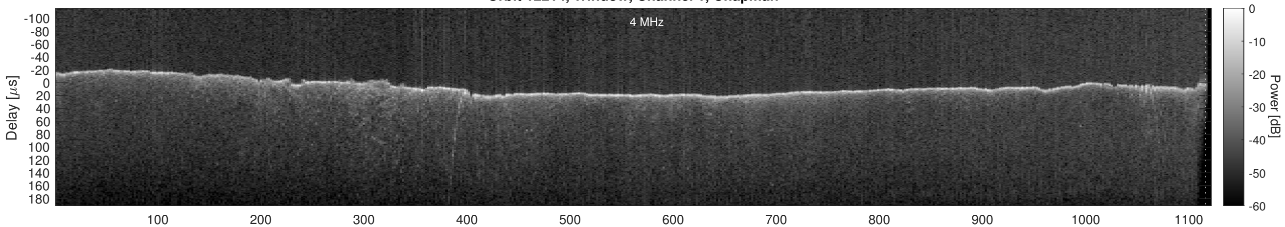
Orbit 12214, Window, Channel 1, Optimized
