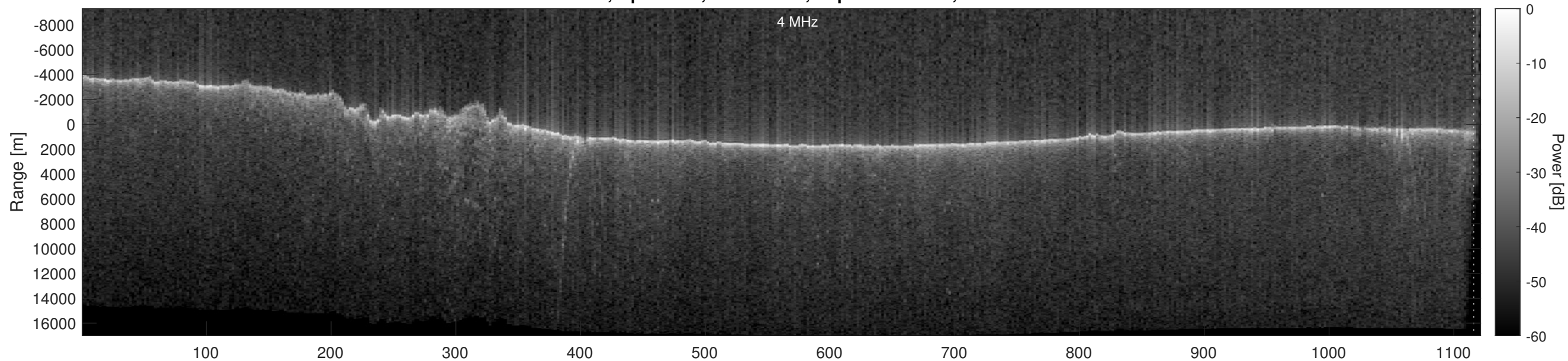
Orbit 12214, Optimized, No Window, Depth-Corrected, Channel 2
