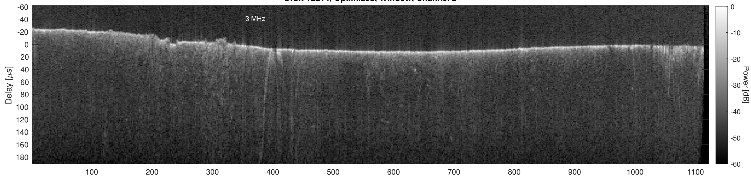
Orbit 12214, Cluttergram
