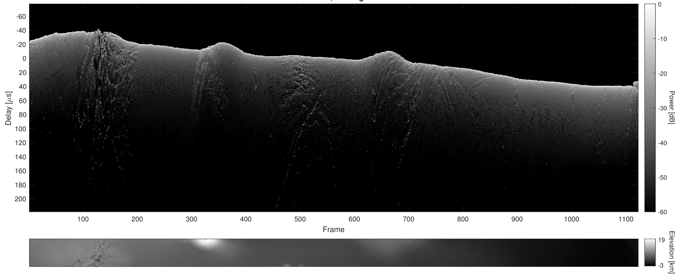
Orbit 12216, Cluttergram
