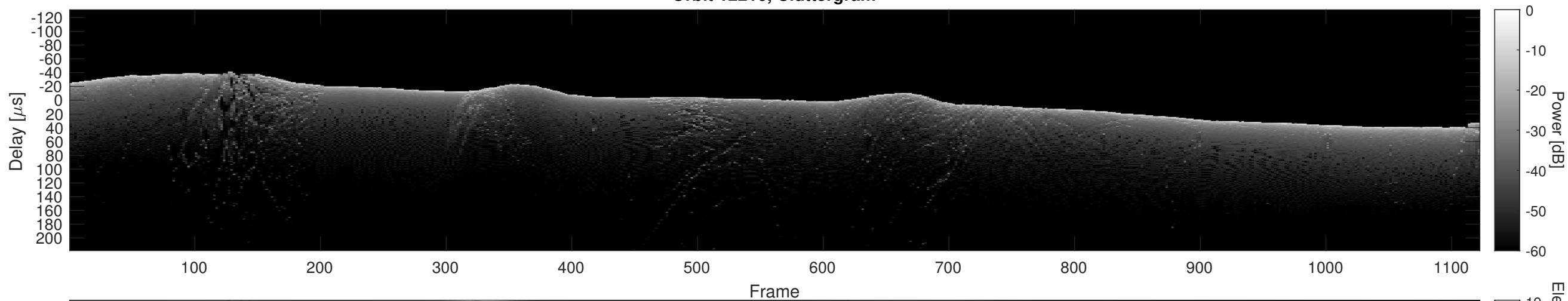
Orbit 12216, Cluttergram
