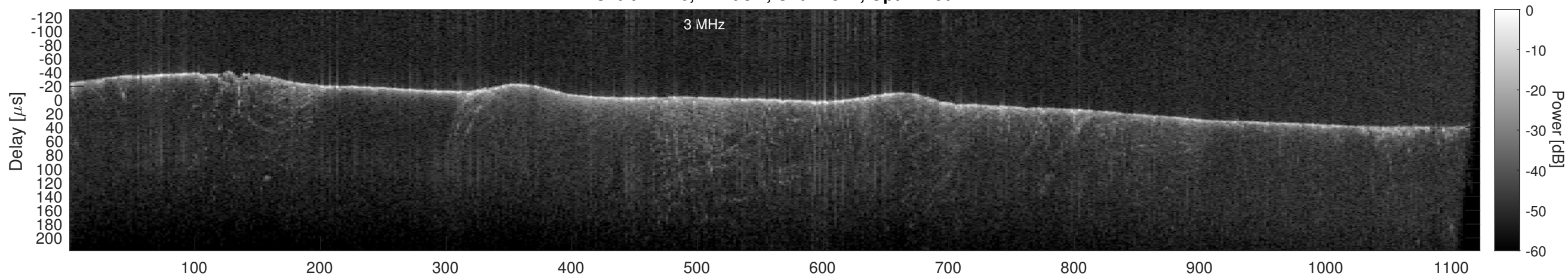
Orbit 12216, Cluttergram
