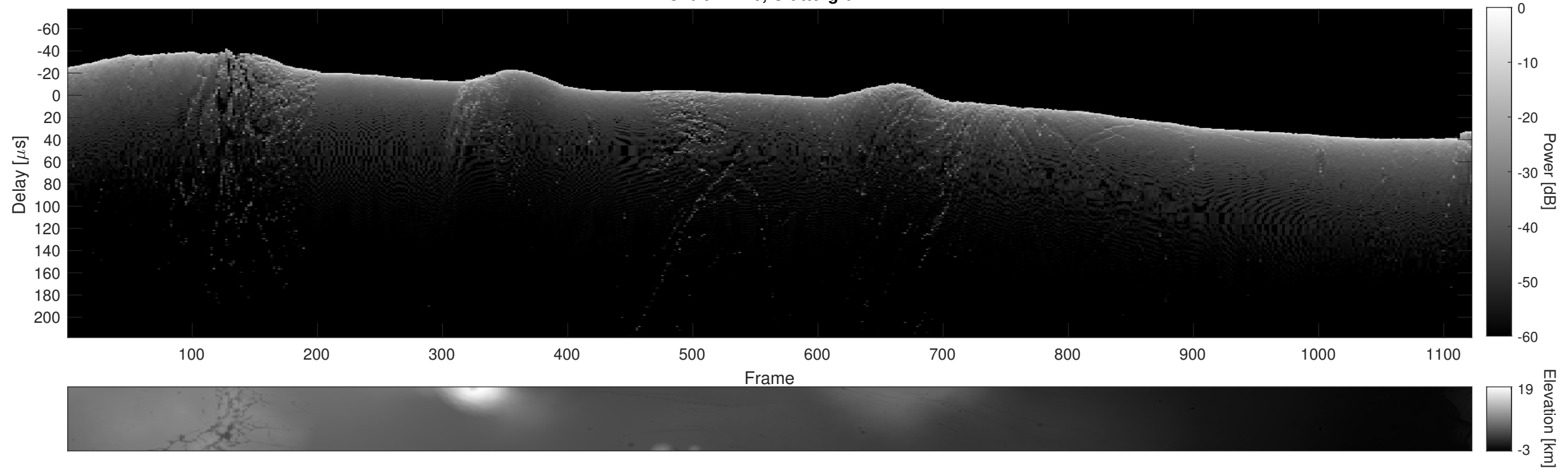
Orbit 12216, Cluttergram
