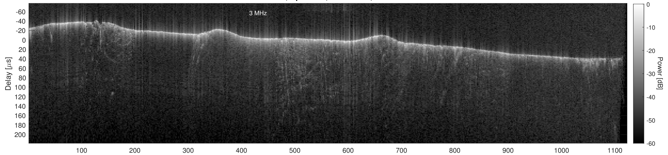
Orbit 12216, Cluttergram
